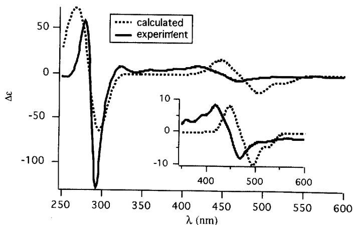
Fig. 7. Calculated and experimental CD-spectrum of \Delta\text{-}[\text{Ru}(\text{bpy})_3]^{2+}
