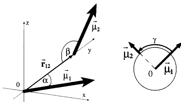
Fig. 4. Coupling of two degenerate transitions with electric dipole moments \mu_1 and \mu_2 .
