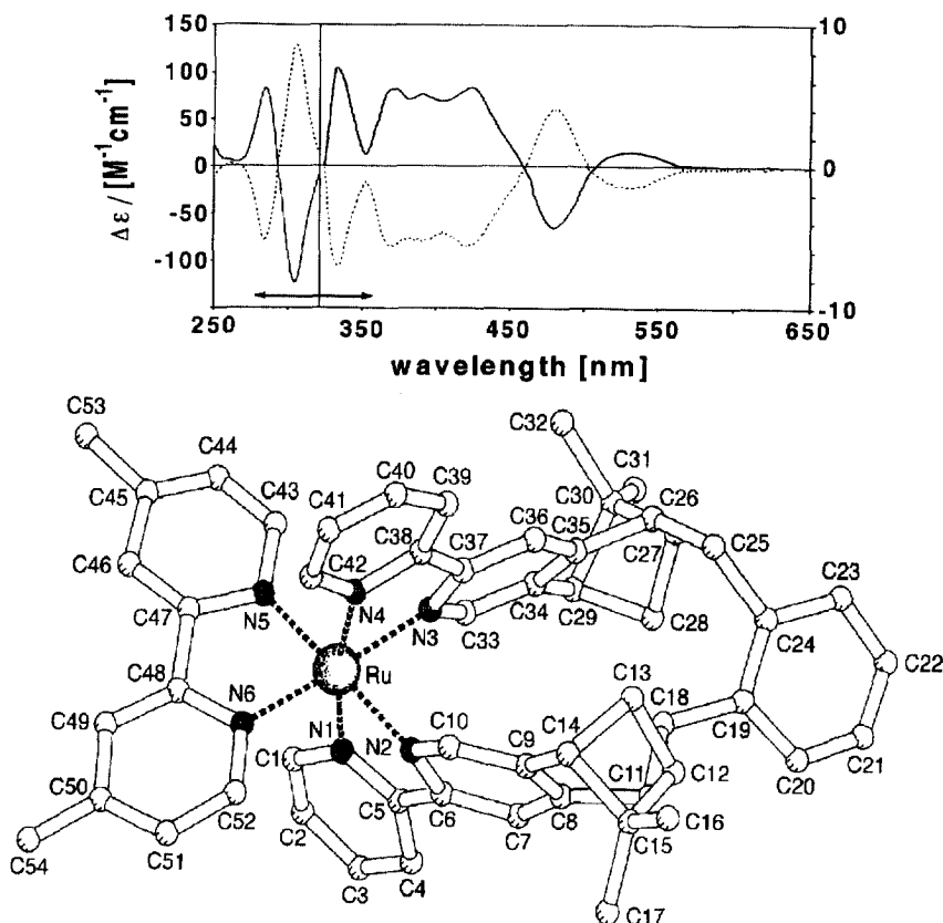
Fig. 3. CD-spectrum and of \Lambda -[Ru((+)-CG[m-xyl])(dmbpy)](PF 6 ) 2 (---) und \Delta -[Ru((-)-CG[m-xyl])(dmbpy)](PF 6 ) 2 (—) in acetonitrile and X-ray structure of the \Delta -form.
