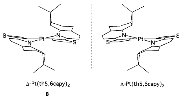
Fig. 9. Enantiomers of \text{Pt}(\text{th}5,6\text{capy})_2 derived from (+)-2-carene and (–)-2-carene.
