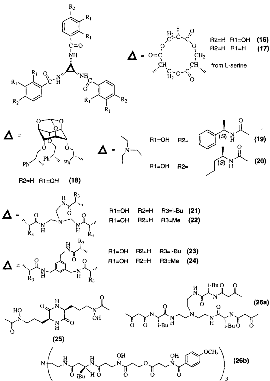
Fig. 14. Enterobactin and related analogues.
