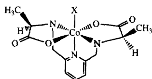
\Delta -[Co(( R,R )-alamp)X] +
