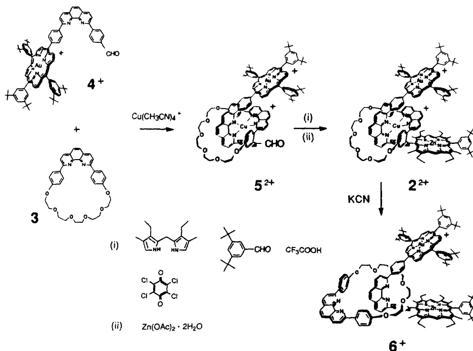
Fig. 4. The key steps leading to [2]-rotaxane 6^+ . (i): (3,3'-diethyl-4,4'-dimethyl-2,2'-dipyrryl)-methane, 3,5-di-tert-butylbenzaldehyde, \text{CF}_3\text{CO}_2\text{H} , \text{CH}_2\text{Cl}_2 , Ar; chloranil, \text{CH}_2\text{Cl}_2 , reflux; (ii) \text{Zn}(\text{OAc})_2 \cdot 2\text{H}_2\text{O} , \text{CHCl}_3/\text{MeOH} reflux.
