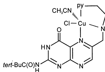
47 (py = 2-pyridyl)
