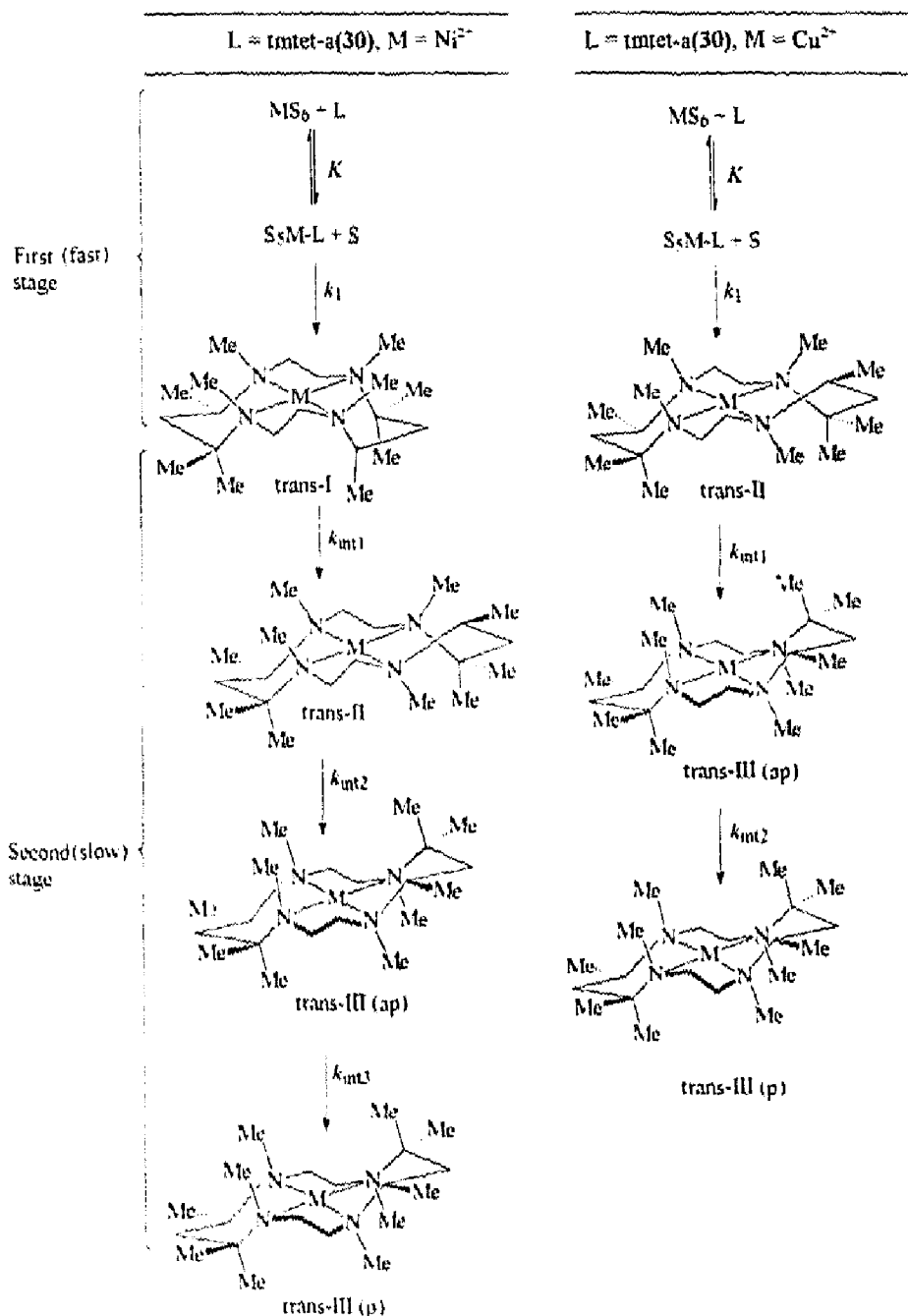
Fig. 2. Reaction scheme suggested for the course of complex formation of ligands 30 with nickel(II) and copper(II) in DMF.
