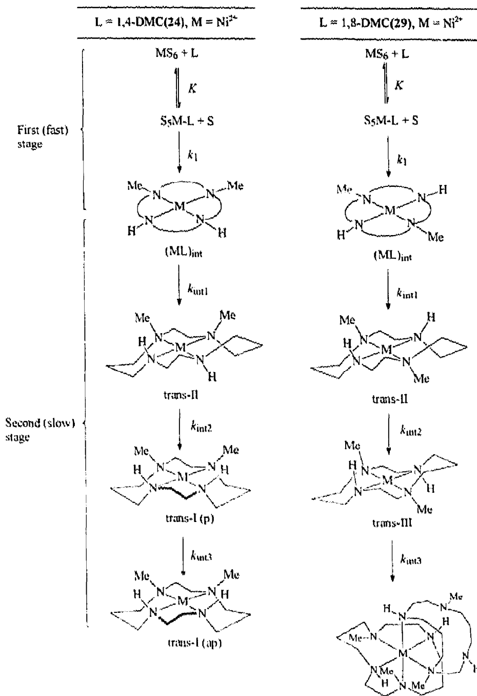
Fig. 1. Reaction scheme suggested for the course of complex formation of ligands 24 and 29 with nickel(II) in DMF.
