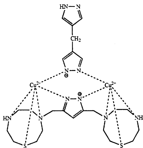
24 [\text{Cu}_2(\text{LH}_1)\text{bispyr}]^{2+}
