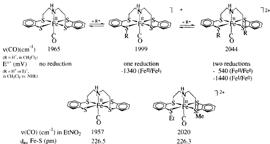
Fig. 2. Electronic, structural, and redox effects in [\text{Fe}(\text{CO})(\text{NHS}_4')] upon reversible protonation ( \text{R} = \text{H}^+ ) or irreversible alkylation ( \text{R} = \text{Me}^+ , \text{Et}^+ ).
