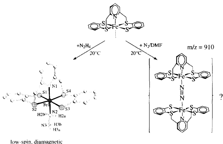
Fig. 7. Sterical enforcement of trans thiolate coordination and Fe(II) low-spin states in [\text{Fe}(\text{'pyS}_4\text{'})] complexes.
