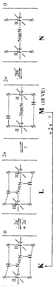
Scheme 4. Redoxisomerism of the [\mu\text{-N}_2\text{H}_2\{\text{Fe}(\text{P}^n\text{Pr}_3)(\text{S}_4')\}_2]^2+ dication.
