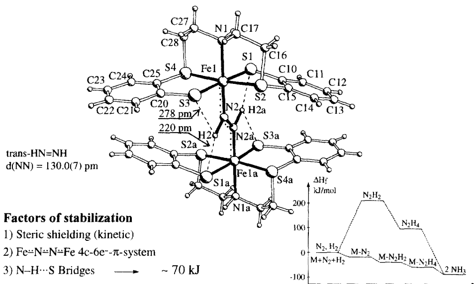
Fig. 3. Molecular structure of [\mu\text{-N}_2\text{H}_2\{\text{Fe}(\text{N}_4\text{S}_4)\}_2] (redrawn after Ref. [33]), factors stabilizing complex-bound \text{N}_2\text{H}_2 , and reaction coordinates for the \text{N}_2 \rightarrow \text{NH}_3 transformation in the absence or presence of suitable metal catalysts.
