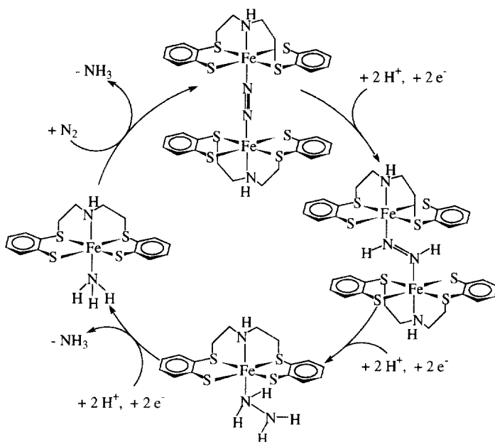
Scheme 3. Hypothetical model cycle of N_2 fixation by [\text{Fe}(\text{N}_4\text{S}_4)] fragments.
