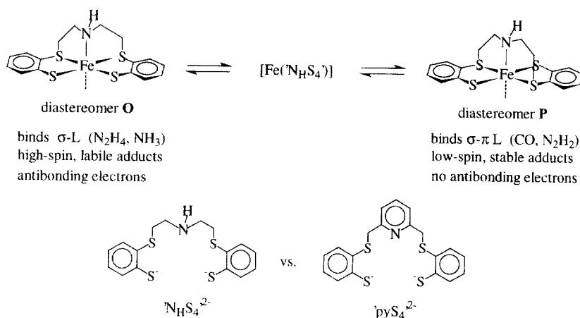
Fig. 6. Diastereoisomerism and low-spin versus high-spin states of [Fe('N_HS_4')] , and schematical drawings of ' N_HS_4 ' 2- and the new ' pyS_4 ' 2- ligand.
