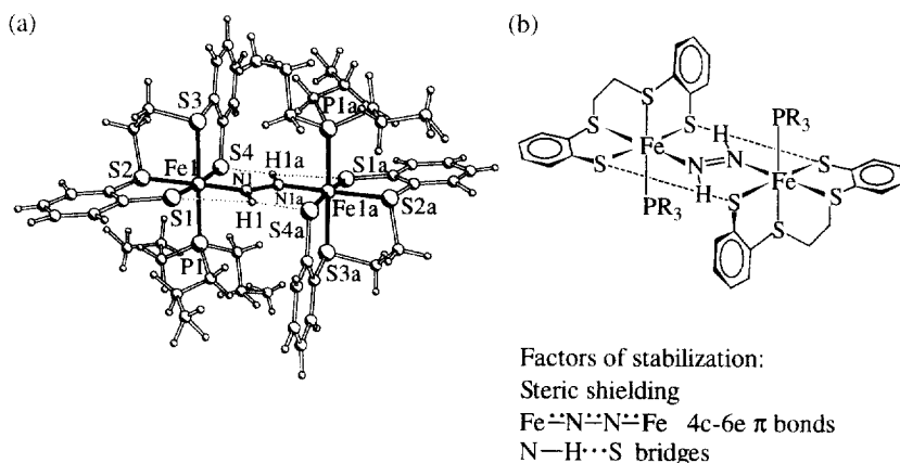
Fig. 4. (a) Molecular structure of [\mu\text{-N}_2\text{H}_2\{\text{Fe}(\text{P''Pr}_3)(\text{'S}_4')\}_2] ; (b) schematical drawing stressing the planar arrangement of Fe centers, thiolate donors and \text{N}_2\text{H}_2 atoms.
