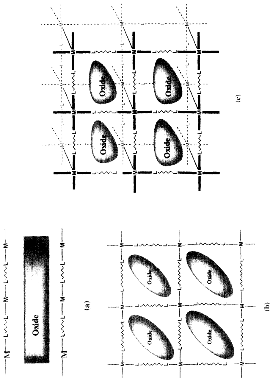
Fig. 6. Schematic views of metal oxide substructures entrained in one-, two-, and three-dimensional coordination complex cation polymers.
