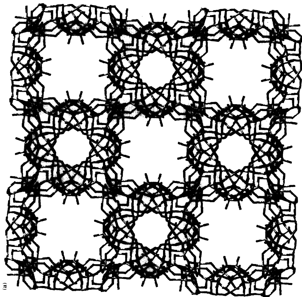
Fig. 3. (a) A view of the complex three-dimensional oxovanadium framework of (\text{H}_3\text{DABCO})\text{K}_{1.33}[\text{V}_6\text{O}_{13}(\text{PO}_4)_2] \cdot x\text{H}_2\text{O} . (b) The pentanuclear fundamental building block of this oxovanadium phosphate framework.
