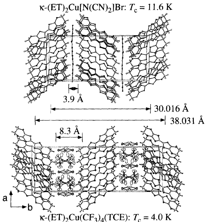
Fig. 6. A comparison of the crystal structures of two \kappa -phase organic superconductors: \kappa\text{-(ET)}_2\text{Cu[N(CN)}_2\text{]Br} and \kappa\text{-(ET)}_2\text{Cu(CF}_3\text{)}_4\text{(TCE)} . The anion layer in \kappa\text{-(ET)}_2\text{Cu(CF}_3\text{)}_4\text{(TCE)} is more than twice as thick as in \kappa\text{-(ET)}_2\text{Cu[N(CN)}_2\text{]Br} . Disorder within the anion layer may result in the lower T_c found in the \kappa\text{-(ET)}_2\text{Cu(CF}_3\text{)}_4\text{(TCE)} salt.
