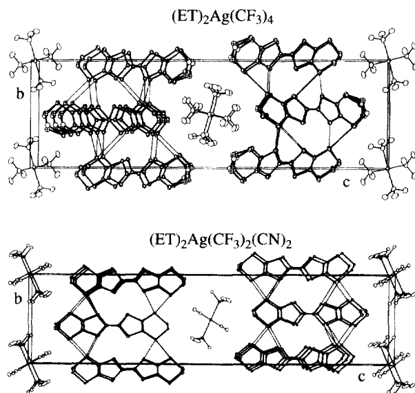
Fig. 3. The top panel depicts a projection of the (\text{ET})_2\text{Ag}(\text{CF}_3)_4 salt on the bc -plane. The lower panel shows a similar projection of the (\text{ET})_2\text{Ag}(\text{CF}_3)_2(\text{CN})_2 structure.
