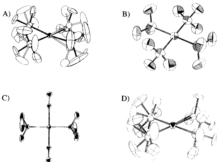
Fig. 4. (A) The disordered M(\text{CF}_3)_4^- anion as crystallized in the \kappa_L-(\text{ET})_2M(\text{CF}_3)_4(1,1,2\text{-trihaloethane}) and \kappa_L-(\text{BEDT-TSF})_2\text{Ag}(\text{CF}_3)_4(\text{TCE}) structures. (B) The ordered M(\text{CF}_3)_4^- anion as crystallized in the (\text{ET})_2M(\text{CF}_3)_4 salts. (C) The \text{Ag}(\text{CF}_3)_2(\text{CN})_2^- anion as crystallized in the (\text{ET})_2\text{Ag}(\text{CF}_3)_2(\text{CN})_2 salt. (D) The \text{Ag}(\text{CF}_3)_3\text{Cl}^- anion as crystallized in the \kappa_L-(\text{BEDT-TSF})_2\text{Ag}(\text{CF}_3)_3\text{Cl}(\text{TCE}) structure.
