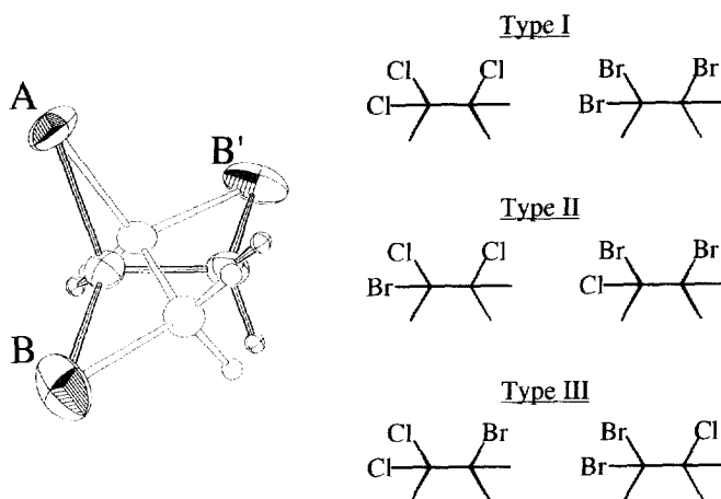
Fig. 7. The disordered solvent molecule in the \kappa_L-(\text{ET})_2\text{M}(\text{CF}_3)_4(1,1,2\text{-trihaloethane}) structures. The halogen positions of the two different orientations of the solvent molecule occupy the corners of the same isosceles triangle. Halogen site A lies on a mirror plane, while sites B and B' are mirror symmetric. The three types of 1,1,2-trihaloethane solvent molecules shown have crystallized into this structural type.
