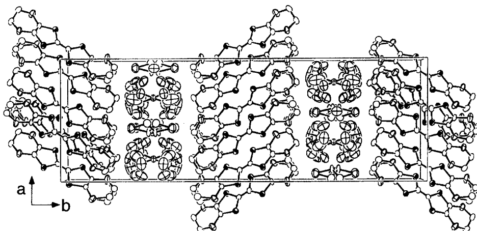
Fig. 9. The crystal structure of \kappa_L -(BEDT-TSF) _2 Ag(CF _3 ) _4 (TCE) illustrated as a projection on the ab -plane.
