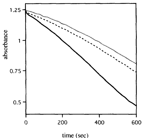
Fig. 7. Decay of ferrocycytochrome c ( 4.5 \times 10^{-5} M) catalyzed by myoglobin ( 1.5 \times 10^{-6} M) in the presence of \text{H}_2\text{O}_2 ( 3.6 \times 10^{-4} M) in 5 mM phosphate buffer (pH 7.0) at 20°C. Solid line corresponds to reconstituted myoglobin rMb(5-Fe); dashed line corresponds to native myoglobin Mb(6-Fe); dotted line corresponds to control experiment in the absence of myoglobin. The decay was monitored at 550 nm.
