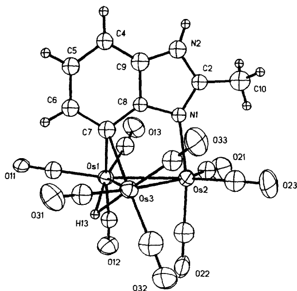
Fig. 3. Solid state structure of [\text{Os}_3(\text{CO})_9(\mu_3\text{-}\eta^2\text{-C}_7\text{H}_4(2\text{-CH}_3)\text{N}_2)(\mu\text{-H})] (9) showing the calculated position of the hydride.
