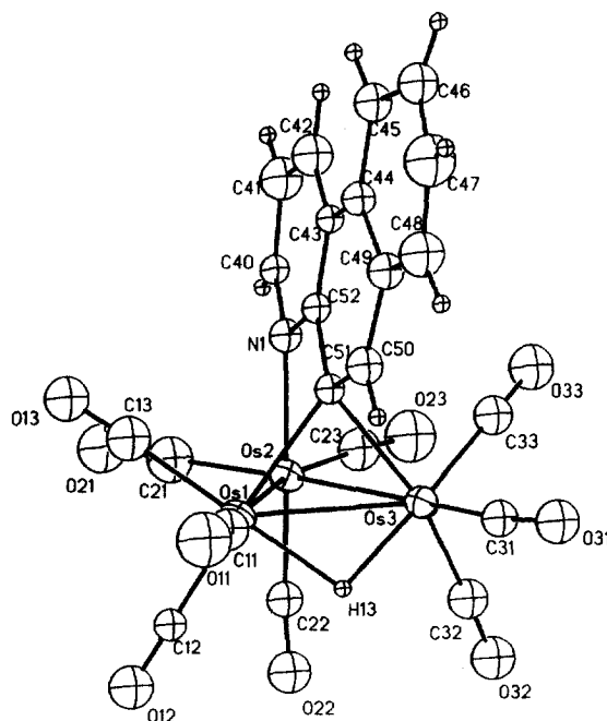
Fig. 2. Solid state structure of [\text{Os}_3(\text{CO})_9(\mu_3\text{-}\eta^2\text{-C}_{13}\text{H}_8\text{N})(\mu\text{-H})] ( 8 ) showing the calculated position of the hydride.
