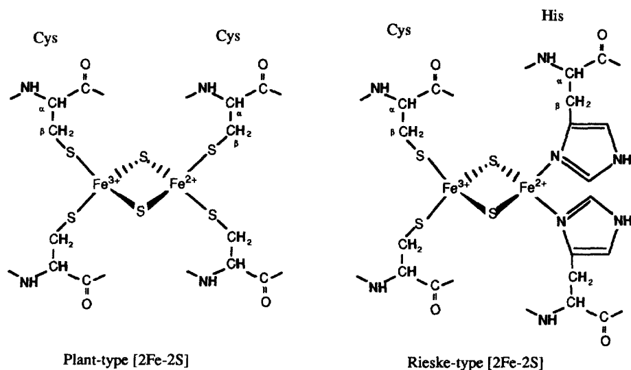
Fig. 1. Covalent structures of the different types of [2\text{Fe-2S}] clusters.
