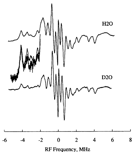
Fig. 4. Solvent-exchangeable protons in c.w. ENDOR spectra of A. platensis [2Fe–2S] ferredoxin.
