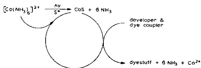
Fig. 15. A photocatalytic image-recording process mediated by light-sensitive cobalt(III) hexammine compounds [\text{Co}(\text{NH}_3)_6]^{3+} [100,102].
