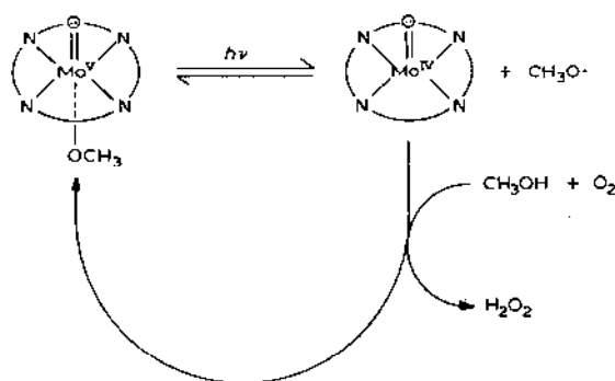
Fig. 6. A simplified scheme of the photoassisted hydrogen peroxide formation mediated by an oxomethoxymolybdenum(V) porphyrin complex [55].
