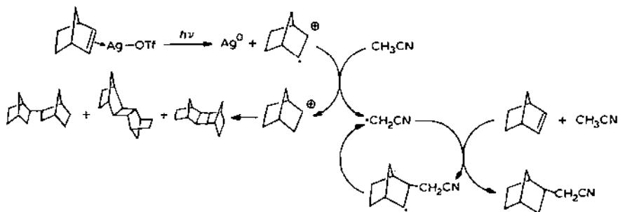
Fig. 10. The photocatalytic reaction of Ag-OTf with norbornene in acetonitrile [76].
