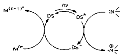
Fig. 18. Indirect dynamic sensitization based on the Oster system [215–217].
