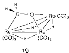
Fig. 15. Structure of [\text{H}_3\text{Re}_3(\mu_3\text{-}\eta^2\text{-CH}_2\text{O})(\text{CO})_9]^{2-} .
