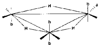
Fig. 1. Structure and ligand arrangements of \text{H}_3\text{Re}_3(\text{CO})_{12} and its derivatives.
