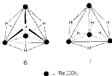
Fig. 7. Structures of H_4Re_4(CO)_{12} and [H_6Re_4(CO)_{12}]^{2-} .
