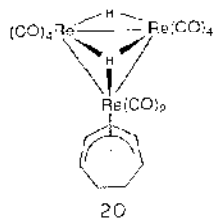
Fig. 16. Structure of \text{H}_2\text{Re}_3(\text{CO})_{10}(\eta^5\text{-C}_7\text{H}_7) .
