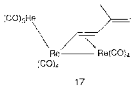
Fig. 13. Structure of \text{Re}_3(\text{CO})_{13}(\mu\text{-}\eta^{1,2}\text{-C}_5\text{H}_7) .
