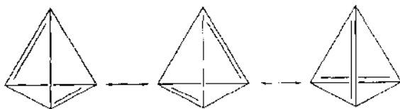
Fig. 6. Proposed hybridization scheme for H_4Re_4(CO)_{12} .
