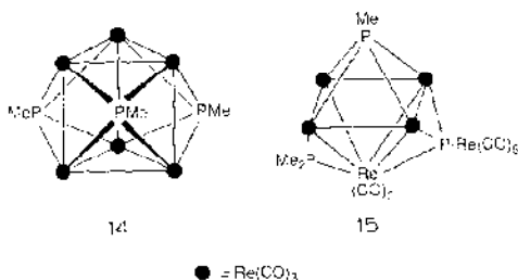
Fig. 11. Structures of \text{Re}_5(\text{CO})_{18}(\mu_2\text{-PMe})_3 and \text{Re}_5(\text{CO})_{14}(\mu_4\text{-PMe})(\mu_3\text{-P}[\text{Re}(\text{CO})_5]) .
