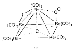
Fig. 9. Structure of [\text{HRe}_5\text{C}(\text{CO})_{16}]^{2-} .
