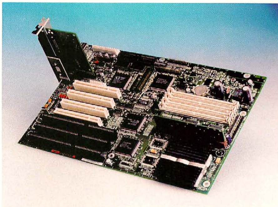
MOTHER OF ALL MOTHERBOARDS The Intel Advanced/EX motherboard's features include: Windows 95 Plug and Play support via the 1MB Intel flash BIOS; built-in Creative Technologies 16-bit stereo Sound Blaster audio; and upgrade capability for forthcoming faster Pentium OverDrive processors.
