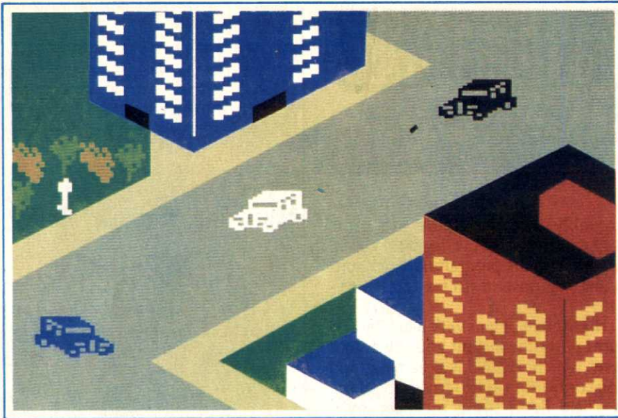
SAFECRACKER (IMAGIC)
