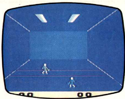
RAQUETBALL (APOLLO)
