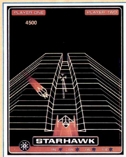
STARHAWK (VECTREX)
