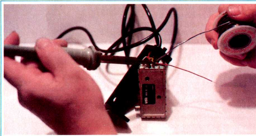
FIGURE 3: Solder one end of the hook-up wire (red wire shown) to the terminal that the yellow wire is connected to.
