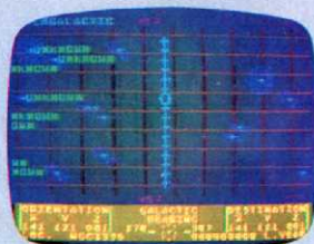
Galactic Starmap Display
