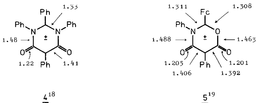
X-ray Data of 4 and 5 ; bond lengths given in Å.
