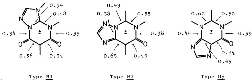
Bond Orders in Bicyclic Mesoionic 4,6-Dioxo-1,5-diazines 17 .
