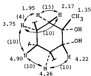
Fig. 1 1 H nmr spectrum of 2 , δ in CDCl 3 at 55°C
