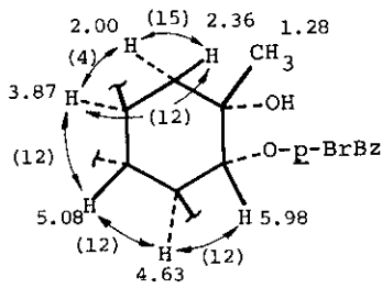
Fig. 2 1 H nmr spectrum of 2 , δ in CDCl 3 at 55°C
