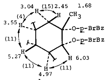
Fig. 3 1 H nmr spectrum of 3 b , δ in CD 3 OD
