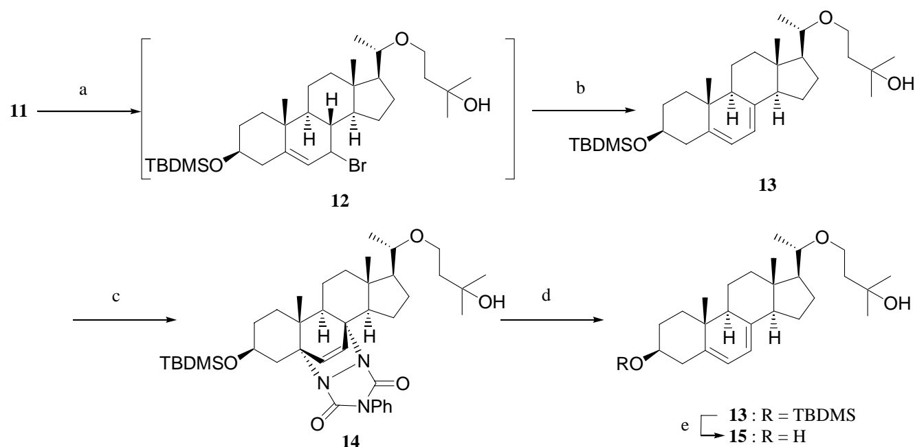
Scheme 2 Reagents and conditions: a) NBS, AIBN (cat.), hexane, reflux. b) \gamma -collidine, toluene, reflux. c) PTAD, \text{CH}_2\text{Cl}_2 , rt. d) DMI, 160 °C. e) TBAF, THF, rt.
