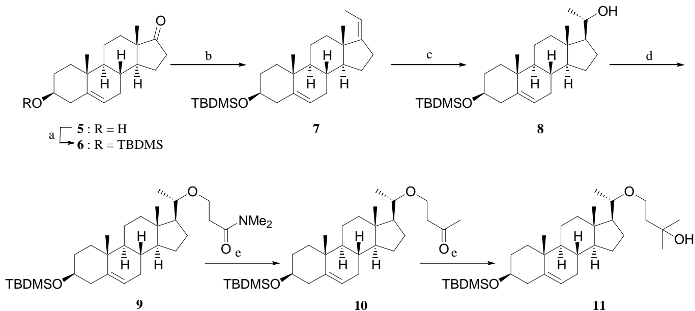
Scheme 1 Reagents and conditions: a) TBDMSCl, imidazole, DMF, rt. b) EtPPh 3 Br, tert -BuOK, THF, 40 °C. c) 9-BBN, THF, rt., 40 °C, then 30% H 2 O 2 -3N NaOH, 0 °C. d) N,N -dimethylacrylamide, THF, 0 °C. e) MeMgBr-CeCl 3 , THF, -10 °C.
