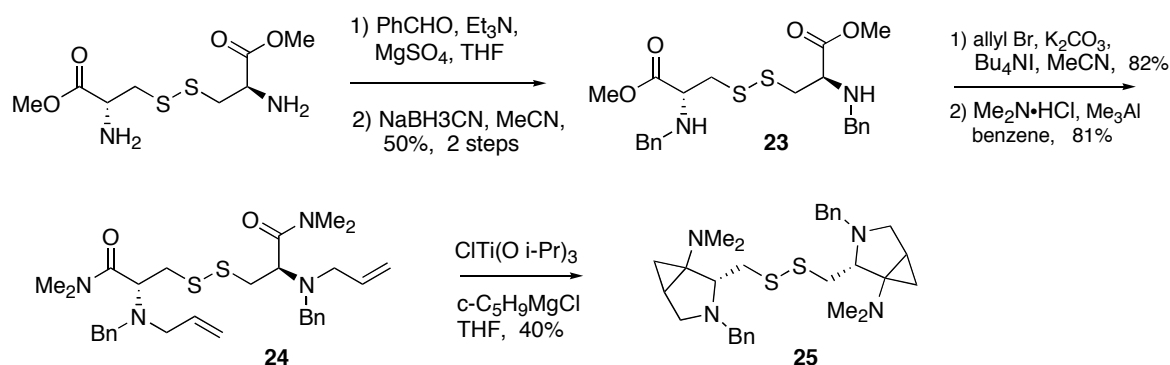
Scheme 5. L-Cystine-derived bicycle.
