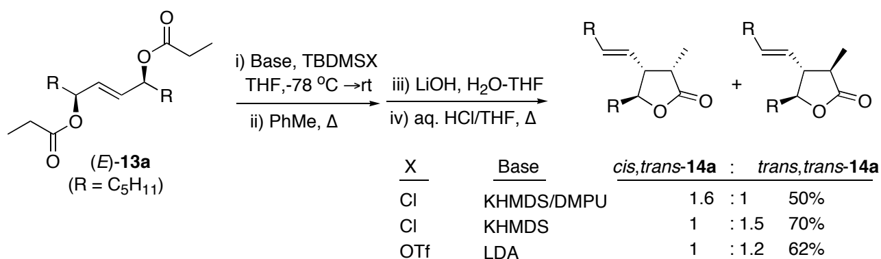
Scheme 8
