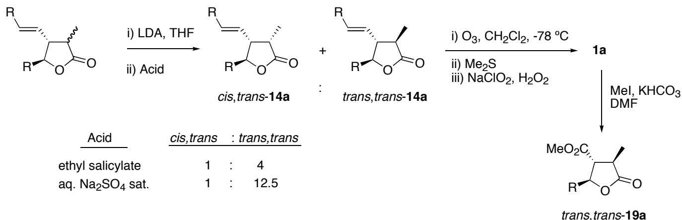
Scheme 9
