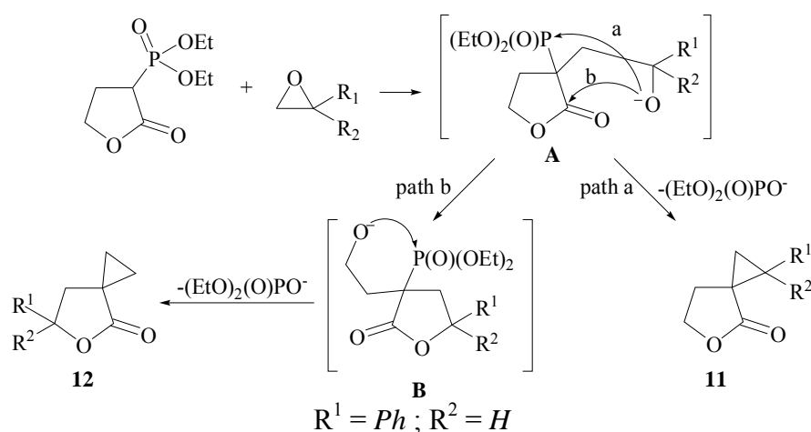
Scheme 3. Reaction of \alpha -phosphono- \gamma -butyrolactone carbanion with 2-phenyloxirane. 2b
