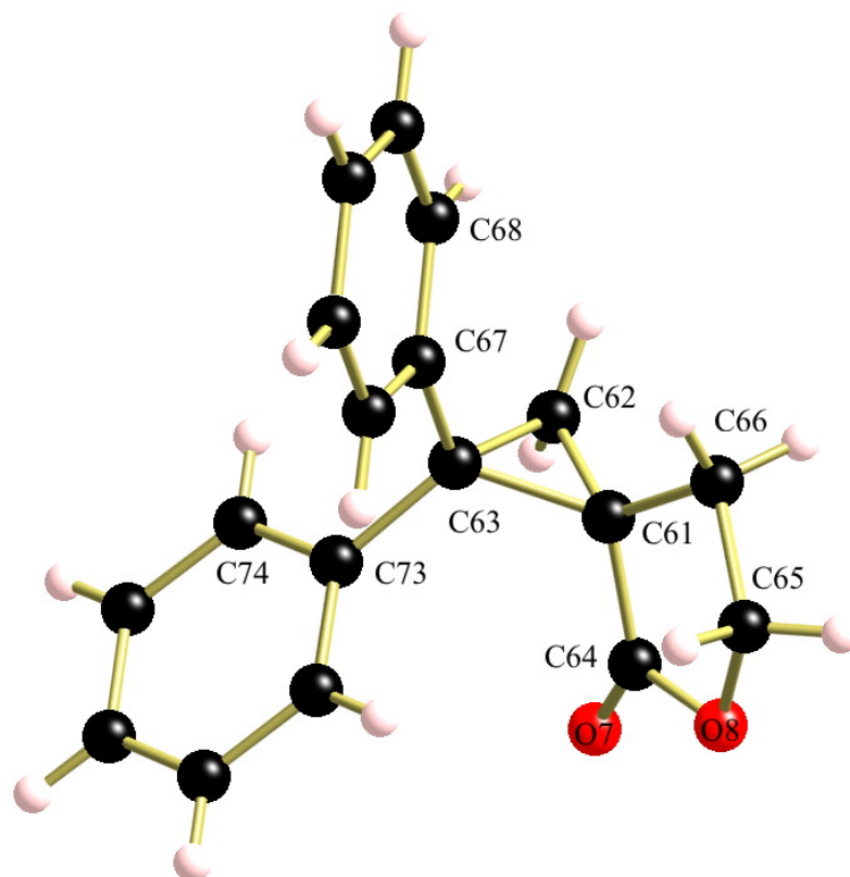
Figure 2. View of the crystal structure of (8b). One of the four independent molecules present in asymmetric unit is shown. The mean values of four equivalent bonds are given in square brackets. Selected bond lengths [Å]: C(61)–C(62) 1.508(3) [1.507], C(61)–C(63) 1.551(3) [1.545], C(62)–C(63) 1.504(3) [1.505], C(61)–C(64) 1.478(3) [1.481], C(61)–C(66) 1.512(3) [1.507], C(64)–O(7) 1.206(3) [1.207], C(64)–O(8) 1.356(3) [1.360].
