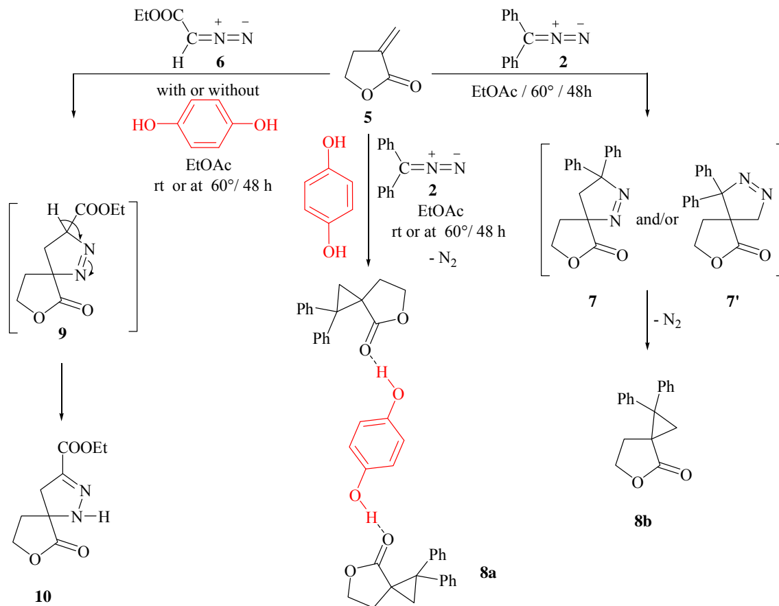
Scheme 2. [3+2] Cycloaddition mechanism of the diazoalkanes ( 2 ) and ( 6 ) towards ( 5 ).
