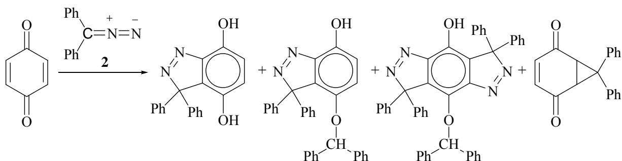
Scheme 4. [3+2] Cycloaddition of benzoquinone and diphenyldiazomethane (in refluxing benzene). 18
