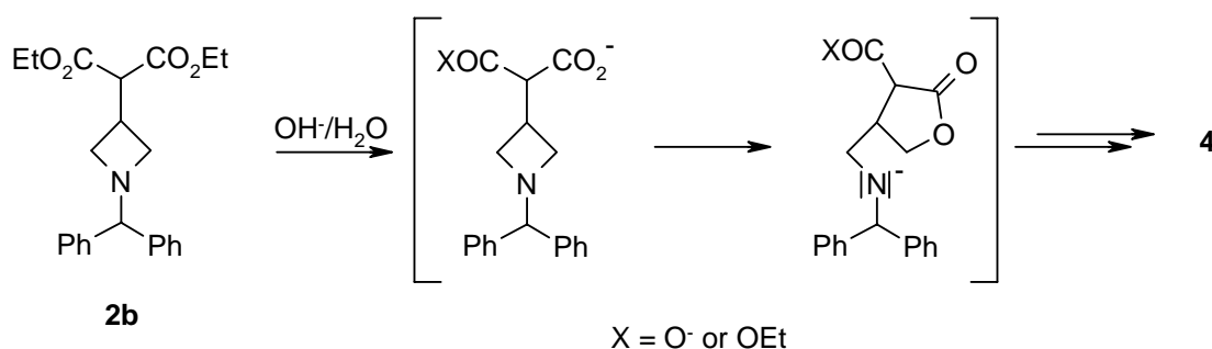
Scheme 5. Postulated mechanism for the formation of lactone derivative 4
