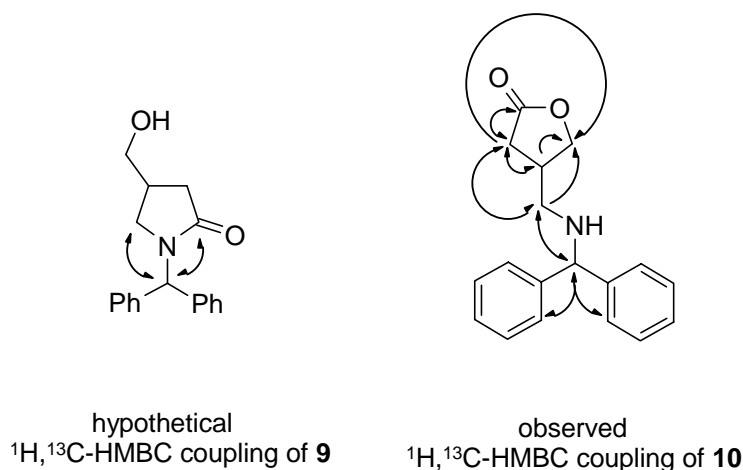
Scheme 4. Expected and observed ^1\text{H},^{13}\text{C} -HMBC couplings for compounds 9 and 10 , respectively.
