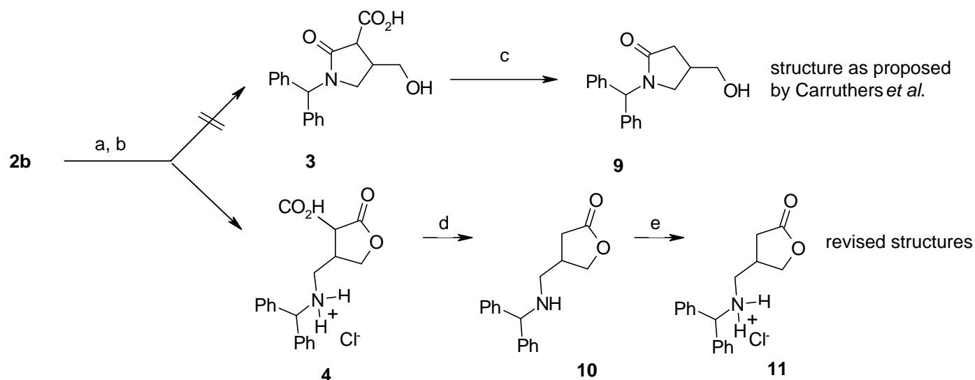
Scheme 3. a KOH, EtOH, H 2 O b acidification to pH 4.5 (1 M HCl) c 130 °C, 2 x 10 -3 bar, 120 min d (1) 130 °C, 2 x 10 -3 bar, 2 h; (2) CC ( n -heptane/EtOAc = 80/20 + 0.5% ethyldimethylamine) e HCl
