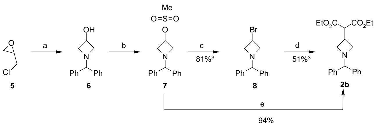
Scheme 2. a Ph 2 CHNH 2 , MeOH b MsCl, pyridine c LiBr, Li 2 CO 3 , THF d,e NaH, CH 2 (CO 2 Et) 2
