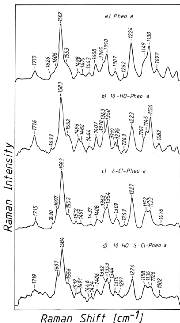
Figure 6. RR spectra of Pheo a derivatives in \text{Et}_2\text{O} with 413.2\text{ nm} excitation. Pheo concentration was approximately 1\text{ mM} for all samples. Laser power, 15\text{ mW} .
