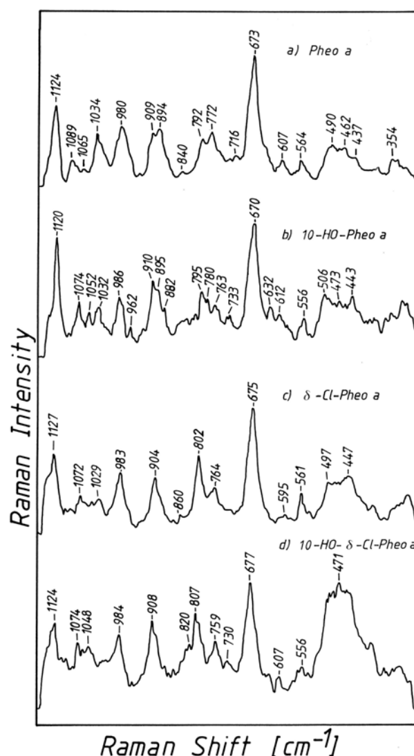
Figure 7. RR spectra (low frequency region) of Pheo a derivatives in \text{Et}_2\text{O} with 413.2\text{ nm} excitation. Pheo concentration was approximately 1\text{ mM} for all samples. Laser power, 15\text{ mW} .
