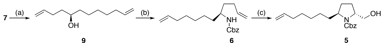
Scheme 1
