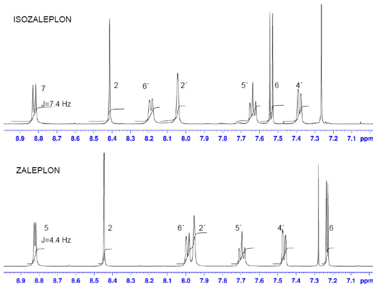
Figure 1 Comparison of aromatic regions of proton spectra for isozaleplon ( 4 ) and zaleplon ( 1 ).
