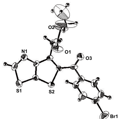
Figure 1. ORTEP drawing of 3I
