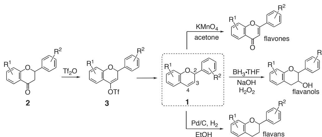
Scheme 1. Transformations of flav-3-ene to several flavonoids
