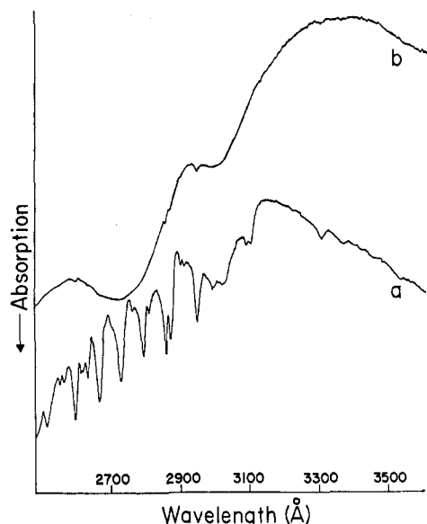
Figure 4.—Electronic spectra of tantalum atoms deposited in a 200:1 Ar:CO matrix: a, original; b, annealed to \sim 30^\circ\text{K} .
