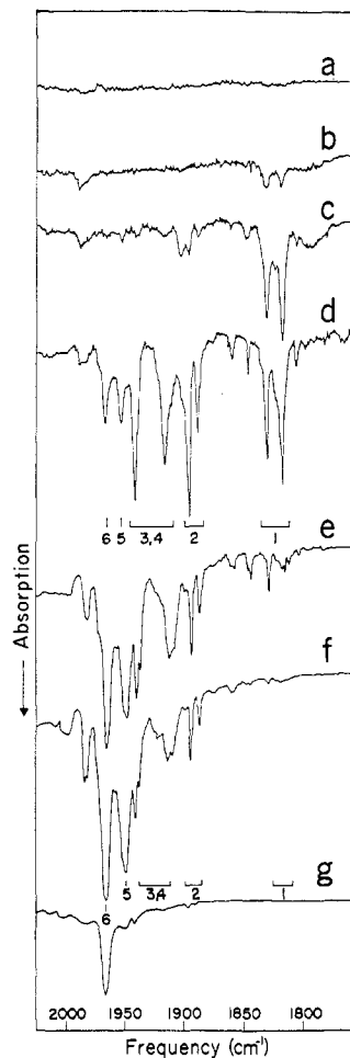
Figure 2.—Infrared spectra of tantalum atoms deposited in a 200:1 Ar:CO matrix and subsequent annealing: a, original; b, 13°K; c, 16°K; d, 18°K; e, 23°K; f, 29°K; g, 35°K (temperatures are relative). The arabic numerals refer to the relative rate of growth and disappearance of the bands.
