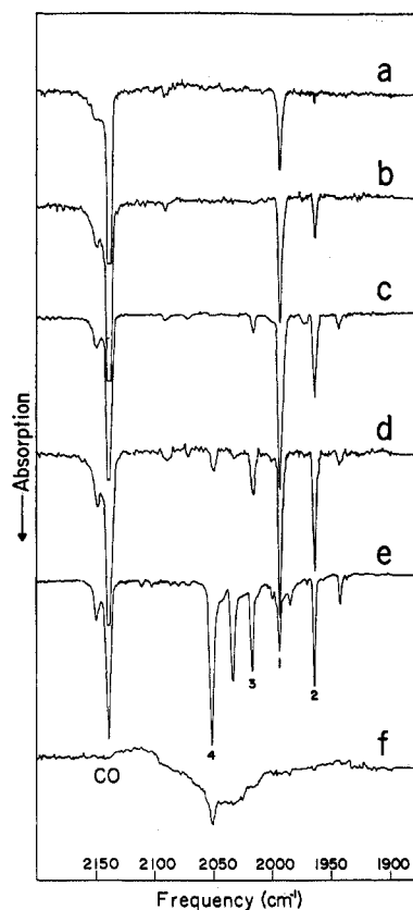
Figure 1.—Infrared spectra of nickel atoms deposited in a 500:1 Ar:CO matrix and subsequent annealing: a, original; b, 17°K; c, 18°K; d, 19°K; e, 26°K; f, 35°K (temperatures are relative). The arabic numerals refer to the relative rate of growth and disappearance of the bands and hence to n in \text{Ni}(\text{CO})_n .
