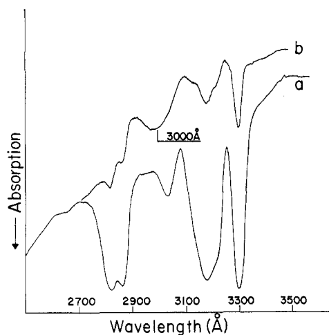
Figure 3.—Electronic spectra of nickel atoms deposited in a 500:1 Ar:CO matrix: a, original; b, annealed to \sim 30^\circ\text{K} .
