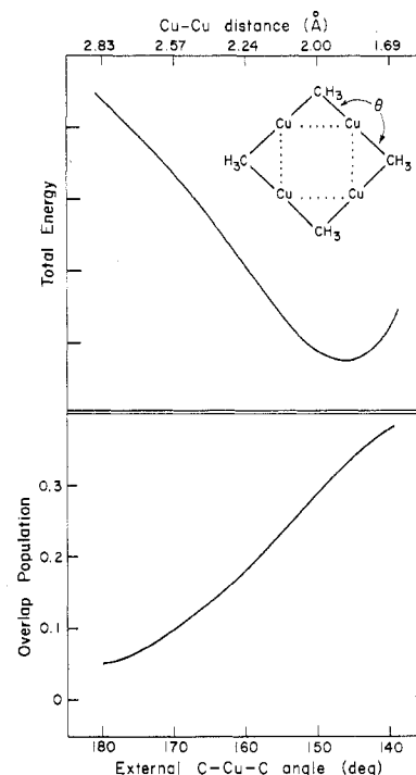
Figure 3. Total energy (top) and Cu-Cu overlap population (bottom) for a (\text{CuCH}_3)_4 tetramer as a function of external C-Cu-C angle. The energy scale markings are in eV.
