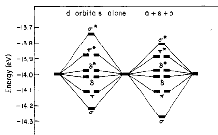
Figure 1. Energy levels of the d block of \text{Cu}_2^{2+} at a separation of 2.58 Å. At left are the results of a calculation with 3d orbitals alone; at right are results for 3d along with 4s and 4p on each center.
