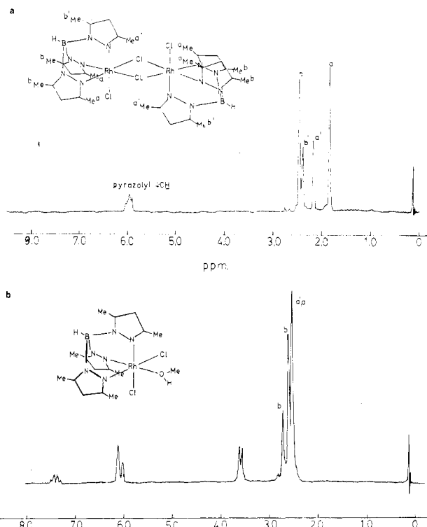
Figure 1. ^1\text{H} NMR spectra of (a) [\text{HB}(3,5\text{-Me}_2\text{pz})\text{RhCl}_2]_2 ( 1 ) and (b) \text{HB}(3,5\text{-Me}_2\text{pz})_3\text{RhCl}_2\text{MeOH} ( 2 ) in \text{CDCl}_3 with \text{Me}_4\text{Si} as an internal reference. The insets are the proposed structures based on ^1\text{H} NMR. The assignments of methyl resonances in both cases are arbitrary.
