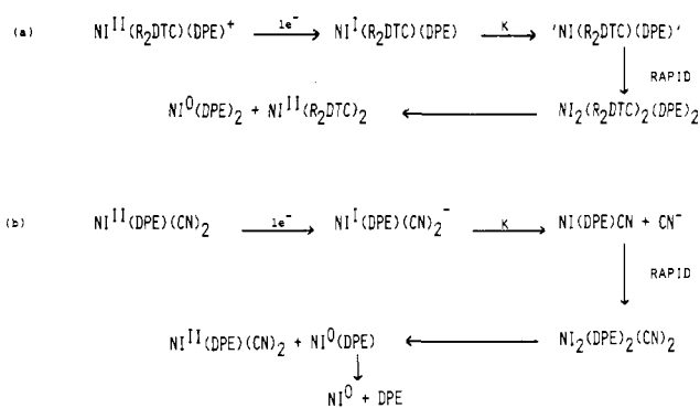
Figure 8. (a) Proposed mechanism of reaction of reduced [\text{Ni}^{\text{II}}(\text{R}_2\text{NCS}_2)(\text{dpe})]^+ . (b) Mechanism of reaction of reduced \text{Ni}^{\text{II}}(\text{dpe})(\text{CN})_2 (ref 31).
