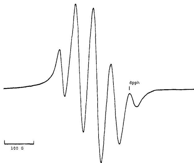
Figure 11. ESR spectrum of [Ni II (dpe) 2 ] + in dichloromethane at -40 °C.
