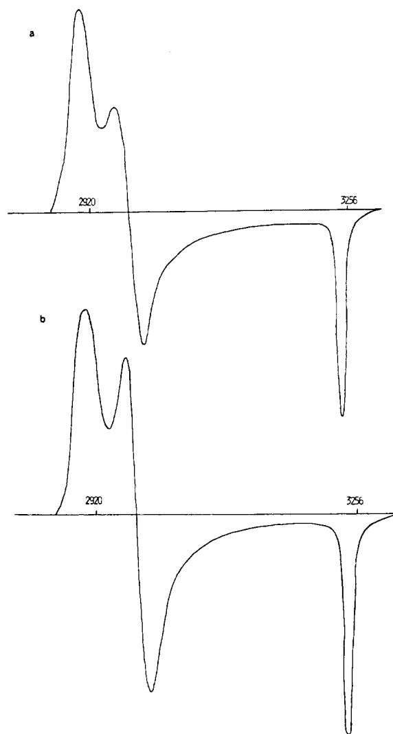
Figure 4. (a) ESR spectrum (9.217 GHz) of reduced \text{Ni}^{\text{II}}(\text{Bu}_2\text{NCS}_2)_2 (species II) in frozen acetone solution (77 K). (b) Simulated ESR spectrum for g values g_x = 2.035 , g_y = 2.207 , and g_z = 2.260 and line widths \sigma_x = 6.0 and \sigma_y = 12.0 G.
