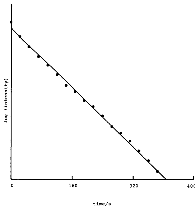
Figure 7. Analysis of the first-order decay of the \text{Ni}^{\text{I}}(\text{Bz}_2\text{NCS}_2)(\text{dpe}) ESR signal in dichloromethane at 0^\circ\text{C} .
