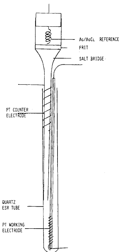
Figure 1. ESR cell for in situ electrolyses.
