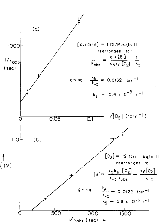
Figure 9. (a) Oxygen and (b) pyridine base dependence of the initial rate of formation of I, R^1 = m -xylylene, R^2 = \text{H} , R^3 = \text{CH}_3 , \text{M} = \text{Fe}^{\text{III}}(\text{py})_2 , from the corresponding \text{Fe}^{\text{II}} complex (monitored at 520 nm, 0.0 °C, in acetone solvent).
