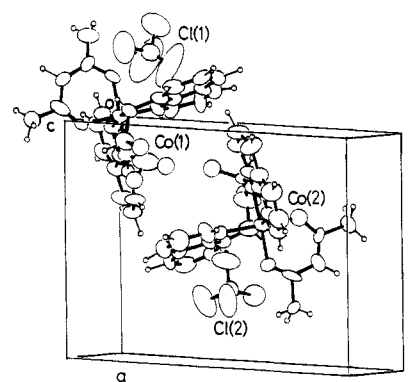
Figure 6. Unit cell structure of [\text{Co}(\text{acac})(R\text{-dqpn}')\text{ClO}_4] projected approximately parallel to the c axis.
