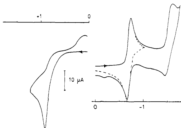
Figure 1. Cyclic voltammetric oxidation and reduction of Ni(BABA)(MNT) (1 mM in 0.1 M TBAP/CH _3 CN) at a 2-mm o.d. Pt disk (scan rate 0.2 V s ^{-1} ; potentials vs. SCE).
