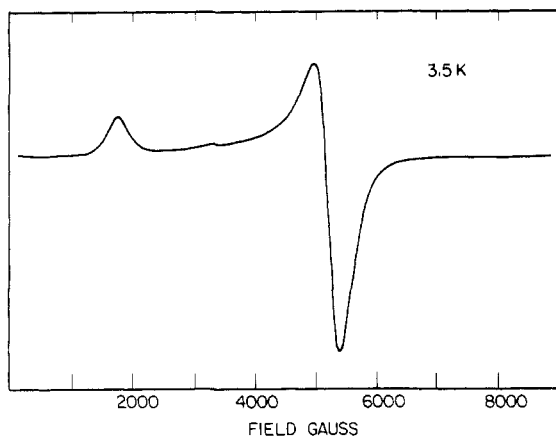
Figure 5. X-Band EPR spectrum of a powdered sample of exo,exo -1,12-dimethyl[1.1]ferrocenophanium triiodide at 3.5 K.
