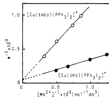
Figure 2. Stern–Volmer relation for the MV 2+ photocatalytic reduction using [Cu(dmp)(PPh 3 ) 2 ] + and [Cu(tmbp)(PPh 3 ) 2 ] + . Reaction conditions: [Cu(dmp)(PPh 3 ) 2 ] + and [Cu(tmbp)(PPh 3 ) 2 ] + = 0.5 × 10 -3 mol/dm 3 ; [PPh 3 ] = 2.5 × 10 -3 mol/dm 3 ; 60:40 v/v ethanol-H 2 O.
