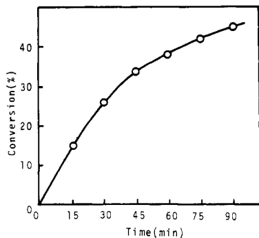
Figure 1. Time-conversion curve (based on the Cu(I) concentration) of MV 2+ reduction photocatalyzed by [Cu(dmp)(PPh 3 ) 2 ] + . Reaction conditions: [Cu(dmp)(PPh 3 ) 2 ] + = 1.0 × 10 -4 mol/dm 3 ; [MV 2+ ] = 1.0 × 10 -3 mol/dm 3 ; [PPh 3 ] = 5.0 × 10 -4 mol/dm 3 ; 60:40 v/v ethanol-H 2 O.
