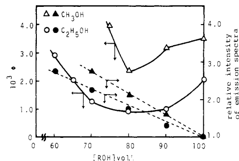
Figure 4. Solvent effect on the MV 2+ photocatalytic reduction and the emission strength of [\text{Cu}(\text{dmp})(\text{PPh}_3)_2]^+ . Reaction conditions: [\text{Cu}(\text{dmp})(\text{PPh}_3)_2]^+ = 0.5 \times 10^{-3} mol/dm 3 ; [\text{PPh}_3] = 2.5 \times 10^{-3} mol/dm 3 ; [\text{MV}^{2+}] = 1.0 \times 10^{-3} mol/dm 3 .
