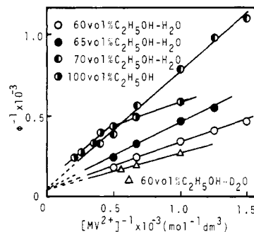
Figure 5. Stern–Volmer relation for the MV 2+ photoreduction catalyzed by [\text{Cu}(\text{dmp})(\text{PPh}_3)_2]^+ in various solvent systems. Reaction conditions are the same as given in Figure 2.
