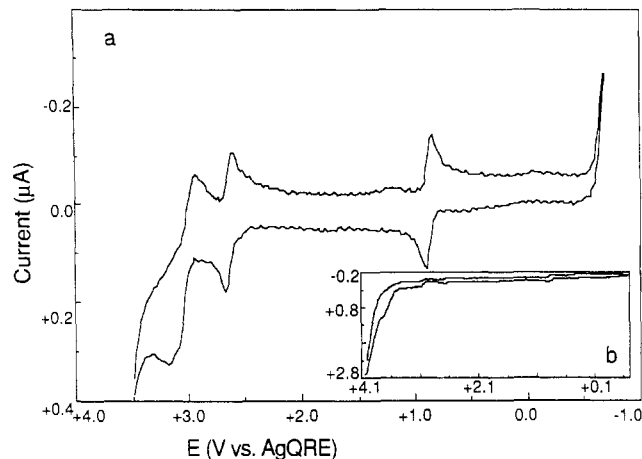
Figure 5. Cyclic voltammogram of 8.0 mM [\text{Ru}(\text{bpy})_3(\text{AsF}_6)_2] in liquid \text{SO}_2 -0.1 M (TBA) \text{AsF}_6 at -70^\circ\text{C} at a 25\text{-}\mu\text{m} Pt electrode. Scan rate: (a) 20 V/s; (b) 10 V/s.
