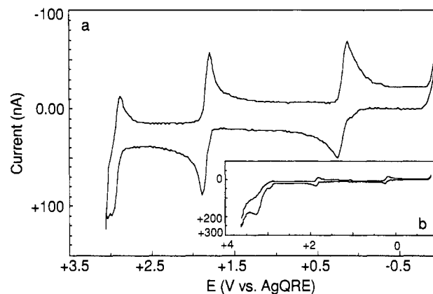
Figure 7. Cyclic voltammogram of 10 mM [\text{Os}(\text{bpy})_3(\text{AsF}_6)_2] in liquid \text{SO}_2/0.1 \text{ M (TBA)AsF}_6 at -70^\circ\text{C} at a 25- \mu\text{m} Pt electrode. Scan rate: (a) 20 V/s, (b) 10 V/s.
