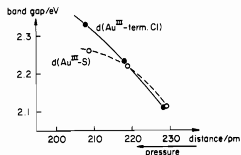
Figure 10. Band gap in 6 as a function of the \text{Au}^{\text{III}} -terminal Cl and \text{Au}^{\text{III}}-\text{S} bond lengths.
