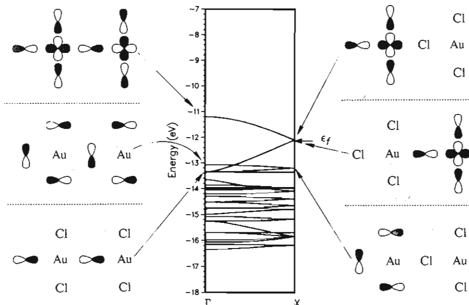
Figure 1. Band-structure diagram for the \{\text{Au}^{\text{II}}\text{Cl}_3\text{-Au}^{\text{II}}\text{Cl}_3\}_n^{2-} chain. The orbital representations are schematic, and only features that will be of importance for the distorted chain are shown.
