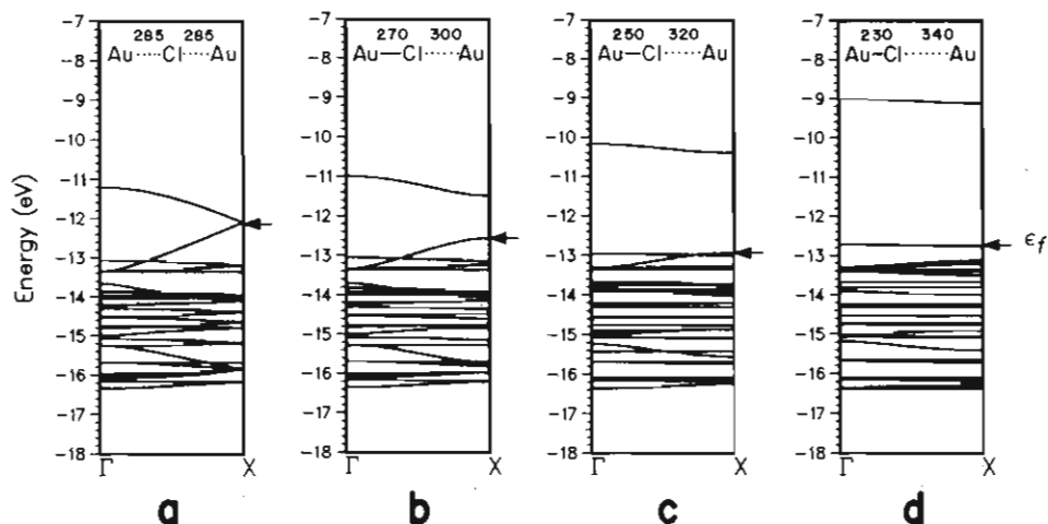
Figure 2. Changes in the band-structure diagram on going from a symmetrical chain (5b) to a localized one (3): (a) \text{Au}^{\text{II}}\text{-Cl} = 285 pm, d = 0 pm ( d = displacement of bridging chlorine from the midpoint between the two golds; see 8); (b) \text{Au}^{\text{III}}\text{-Cl} = 270 pm, d = 15 pm; (c) \text{Au}^{\text{III}}\text{-Cl} = 250 pm, d = 35 pm; (d) \text{Au}^{\text{III}}\text{-Cl} = 230 pm, d = 55 pm.
