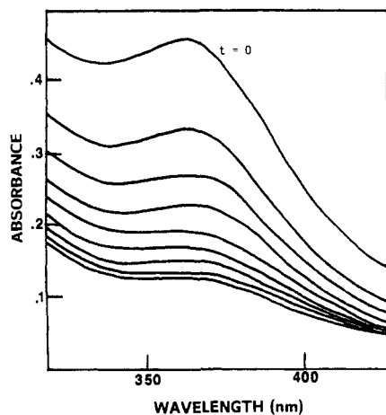
Figure 1. Variation of the UV-vis spectrum of Co(II)-BISBAMP dioxygen complexes with time ( [\text{BISBAMP}]_T = \frac{1}{2}[\text{Co}]_T = 1.98 \times 10^{-4} M; t = 50.0 °C; \mu = 0.10 M \text{KNO}_3 ; \text{p}[\text{H}] = 11.32 ; time intervals = 20 min).
