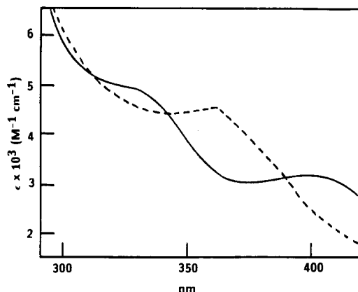
Figure 3. Calculated electronic spectra for Co(II)-BISBAMP dioxygen complexes: \text{Co}_2\text{LO}_2(\text{OH})_2^{2+} (—) and \text{Co}_2\text{LO}_2(\text{OH})_3^+ (---).
