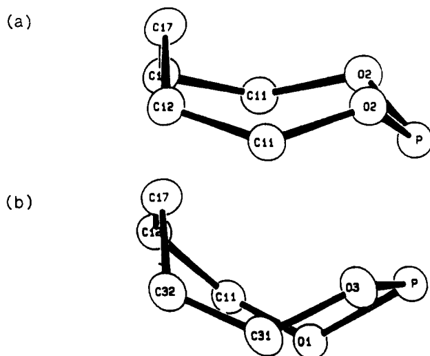
Figure 5. ORTEP plot showing the conformation of the eight-membered ring for (a) \text{CH}_2[(t\text{-Bu})\text{MeC}_6\text{H}_4\text{O}]_2\text{P}(\text{OCH}_2\text{CF}_3)_3 ( 1 ) and (b) \text{CH}_2\text{-(C}_6\text{H}_4\text{O)}_2\text{P}(\text{OCH}_2\text{CF}_3)_3 ( 2 ).
