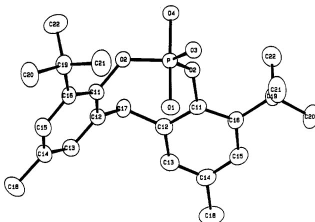
Figure 1. ORTEP plot of \text{CH}_2[(t\text{-Bu})\text{MeC}_6\text{H}_4\text{O}]_2\text{P}(\text{OCH}_2\text{CF}_3)_3 (1) with thermal ellipsoids at the 30% probability level. Atoms with the same label are related by a crystallographic mirror plane. Atoms of the trifluoroethyl groups and hydrogen atoms are omitted for clarity.
