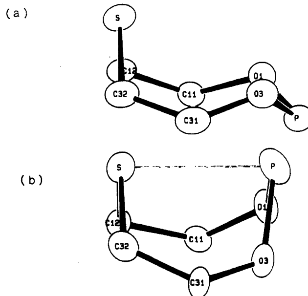
Figure 6. ORTEP plot showing the conformation of the eight-membered ring for (a) \text{S}(\text{Me}_2\text{C}_6\text{H}_4\text{O})_2\text{P}(\text{OCH}_2\text{CF}_3)_3 ( 3 ) and (b) \text{S}[(t\text{-Bu})_2\text{C}_6\text{H}_4\text{O}]_2\text{P}(\text{OCH}_2\text{CF}_3)_3 ( 4 ).
