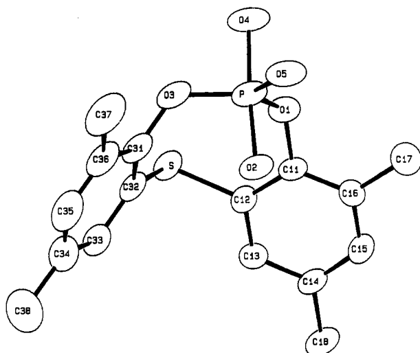
Figure 3. ORTEP plot of \text{S}(\text{Me}_2\text{C}_6\text{H}_2\text{O})_2\text{P}(\text{OCH}_2\text{CF}_3)_3 ( 3 ) with thermal ellipsoids at the 30% probability level. Atoms of the trifluoroethyl groups and hydrogen atoms are omitted for clarity.
