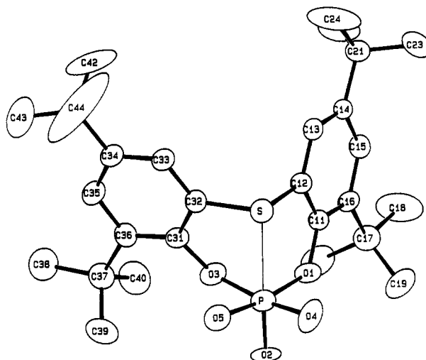
Figure 4. ORTEP plot of \text{S}[(t\text{-Bu})_2\text{C}_6\text{H}_2\text{O}]_2\text{P}(\text{OCH}_2\text{CF}_3)_3 ( 4 ) with thermal ellipsoids at the 30% probability level. Atoms of the trifluoroethyl groups and hydrogen atoms are omitted for clarity.
