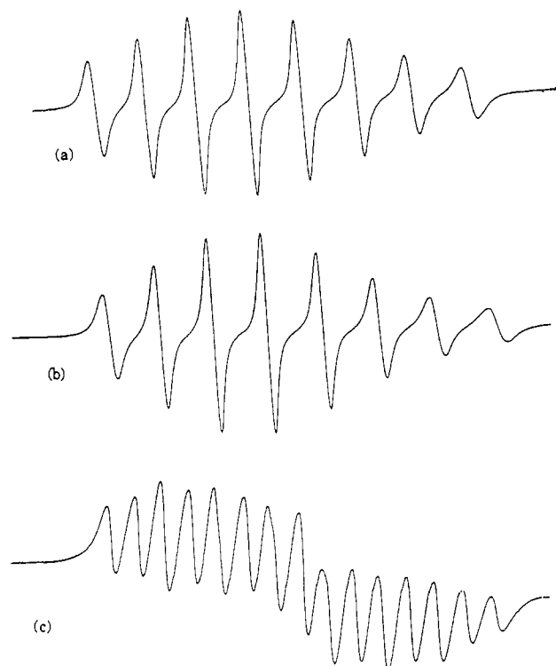
Figure 6. Fluid-solution ESR spectra of (a) [[\text{HB}(\text{Me}_2\text{pz})_3]\text{VOCl}(\text{Me}_2\text{pzH})] (I), (b) [[\text{HB}(\text{Me}_2\text{pz})_3]\text{VO}(\text{benzoate})(\text{Me}_2\text{pzH})] (II), and (c) [[\text{HB}(\text{Me}_2\text{pz})_3]\text{VO}(\mu\text{-malonate})\text{VO}(\text{Me}_2\text{pzH})\{\text{HB}(\text{Me}_2\text{pz})_3\}] (III), in dichloromethane at X-band frequency. Scan range: 1000 G.
