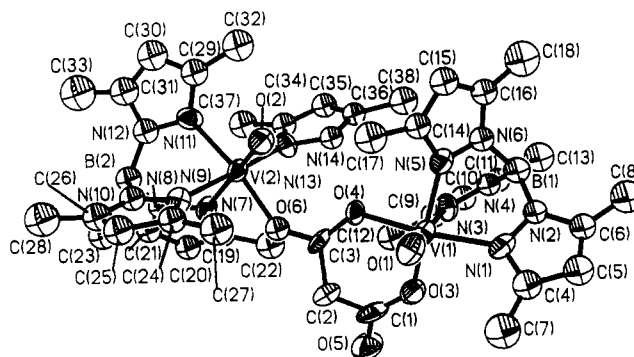
Figure 3. Structure of [[\text{HB}(\text{Me}_2\text{pz})_3]\text{VO}(\mu\text{-malonate})\text{VO}(\text{Me}_2\text{pzH})\{\text{HB}(\text{Me}_2\text{pz})_3\}] (III), shown by an ORTEP diagram with 50% probability thermal ellipsoids and the atom-numbering scheme.
