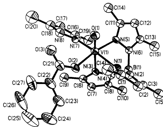
Figure 2. Structure of [[\text{HB}(\text{Me}_2\text{pz})_3]\text{VO}(\text{benzoate})(\text{Me}_2\text{pzH})] (II), shown by an ORTEP diagram with 50% probability thermal ellipsoids and the atom-numbering scheme.
