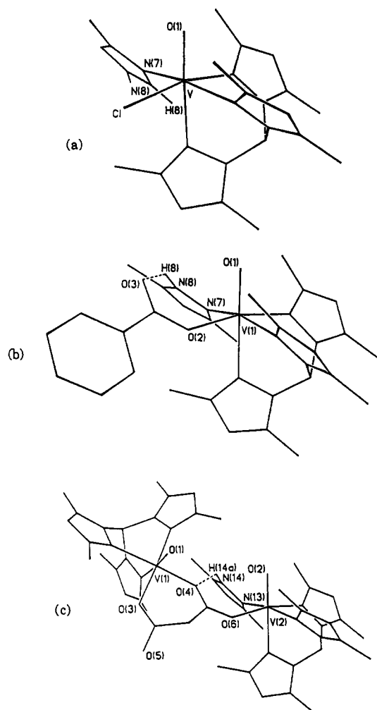
Figure 4. Line drawings of (a) [\{\text{HB}(\text{Me}_2\text{pz})_3\}\text{VOCl}(\text{Me}_2\text{pzH})] (I), (b) [\{\text{HB}(\text{Me}_2\text{pz})_3\}\text{VO}(\text{benzoate})(\text{Me}_2\text{pzH})] (II), and (c) [\{\text{HB}(\text{Me}_2\text{pz})_3\}\text{VO}(\mu\text{-malonate})\text{VO}(\text{Me}_2\text{pzH})\{\text{HB}(\text{Me}_2\text{pz})_3\}] (III), showing the stereochemistry at the vanadium atom and intramolecular hydrogen-bonding interactions.
