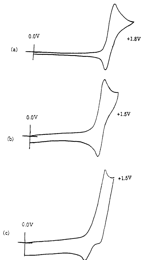
Figure 5. Cyclic voltammograms of (a) [[\text{HB}(\text{Me}_2\text{pz})_3]\text{VOCl}(\text{Me}_2\text{pzH})] (I), (b) [[\text{HB}(\text{Me}_2\text{pz})_3]\text{VO}(\text{benzoate})(\text{Me}_2\text{pzH})] (II), and (c) [[\text{HB}(\text{Me}_2\text{pz})_3]\text{VO}(\mu\text{-malonate})\text{VO}(\text{Me}_2\text{pzH})\{\text{HB}(\text{Me}_2\text{pz})_3\}] (III), in dichloromethane. Peak separations (at -20^\circ\text{C} ), \Delta E and I_p^A/I_p^C : (I) 126 mV, 1.12; (II) 94 mV, 1.13; (III) 86 mV, 0.2. For ferrocene under the same conditions E_{1/2} = 0.430 V, \Delta E = 75 mV, and I_p^A/I_p^C = 1.05 .
