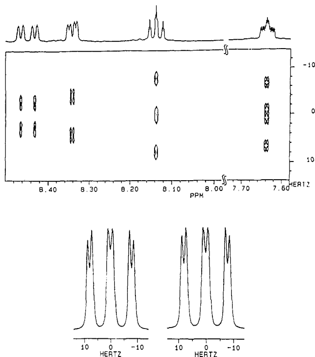
Figure 7. 2D homonuclear J -resolved NMR spectrum at 500 MHz in the aromatic region for complex 4 . The two multiplets in the bottom part of the figure are the two barely-resolved resonances in the \approx 8.14 ppm region.
