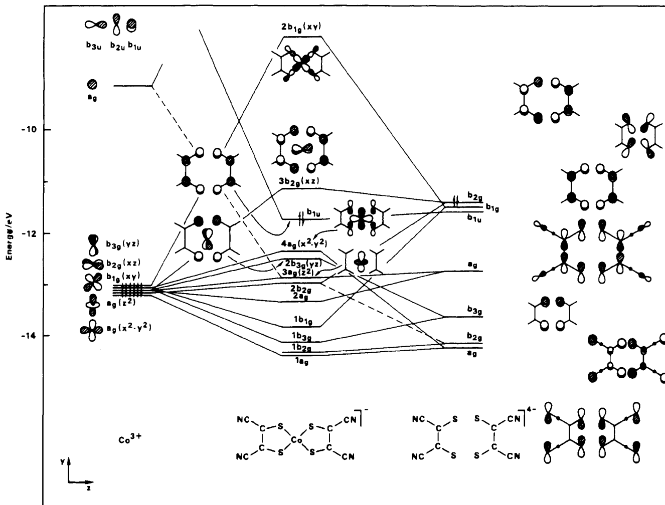
Figure 6. Interaction diagram for Co(III) and two mnt ligands.
