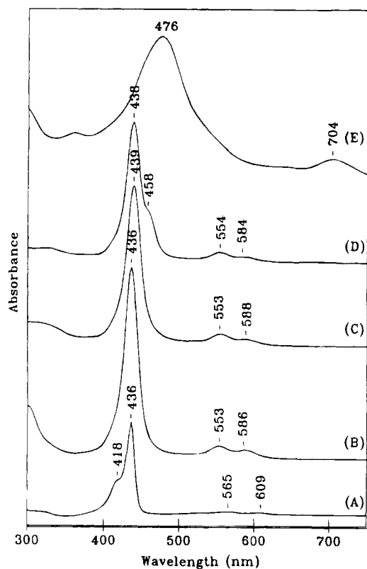
Figure 3. UV-visible absorption spectra of (A) NiTPP, (B) NiOHETPP (Ni5), (C) NiOATPP (Ni4), (D) NiOATPP-OME (Ni3), and (E) NiOATNPP-OME (Ni6) in coordinating solvent. Spectra of (1-5) \times 10^{-4} M solutions were obtained in 1-methylimidazole. Baselines in the individual spectra have been arbitrarily shifted for clarity.
