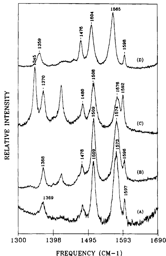
Figure 5. Resonance Raman spectra of (A) NiOAATPP, (B) NiOAATPP-OME, (C) NiOAATNPP-OME, and (D) NiOHETPP. Solvent for porphyrin solution was either methylene chloride or acetone, and 413.1-nm laser excitation was used for obtaining Raman spectra.
