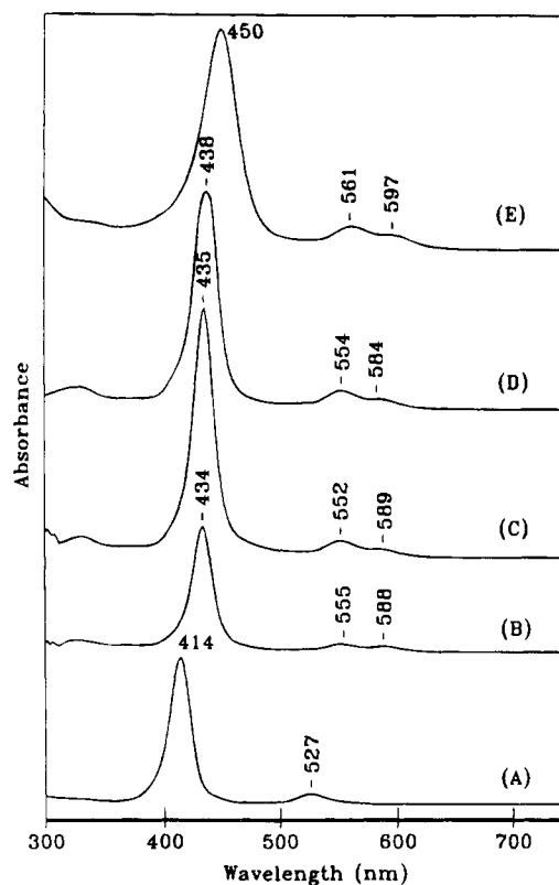
Figure 2. UV–visible absorption spectra of four-coordinate (A) \text{NiTPP} , (B) \text{NiOHETPP} ( Ni5 ), (C) \text{NiOAAATPP} ( Ni4 ), (D) \text{NiOAAATPP-OME} ( Ni3 ), and (E) \text{NiOAAATNPP-OME} ( Ni6 ). Spectra of (1-5) \times 10^{-4}\text{ M} solutions were obtained in either neat methylene chloride or acetone. Baselines in the individual spectra have been arbitrarily shifted for clarity.
