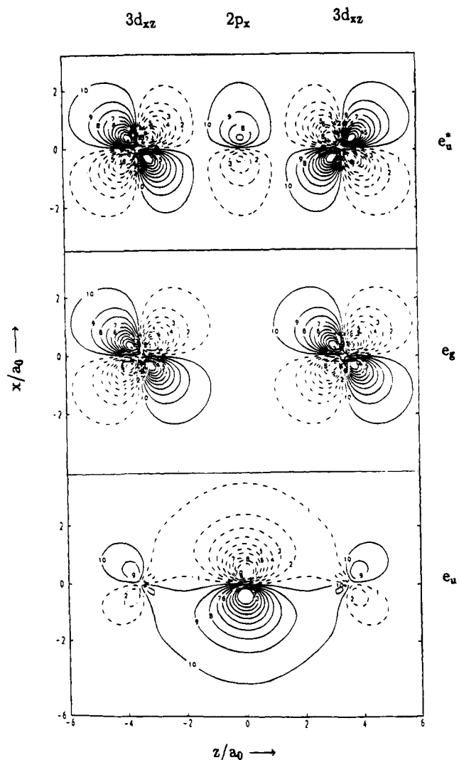
Figure 2. Contour plots of the valence orbitals e_{ux} , e_{gx} , e_{ux}^* of the L_5Cr-O-CrL_5 complex.
