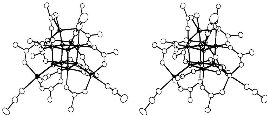
Figure 2. Stereoview of complex 1b.
