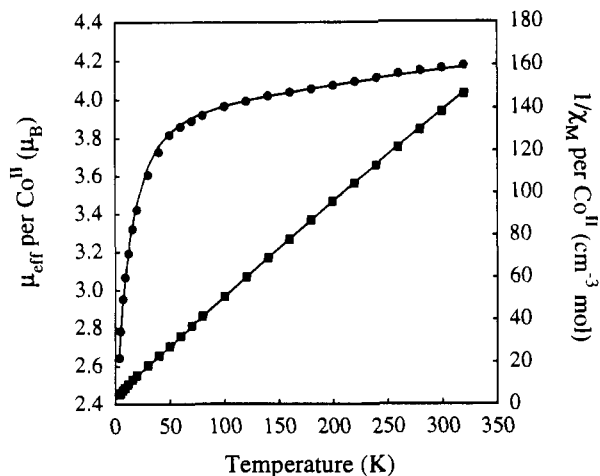
Figure 4. Plots of effective magnetic moment, \mu_{\text{eff}}/\text{Co}^{\text{II}} (●), and the reciprocal of the molar magnetic susceptibility per \text{Co}^{\text{II}} , 1/\chi_{\text{M}} (■), versus temperature. The solid lines are derived from fits of the \chi_{\text{M}} vs T data in the 4–320 K range to eq 2. See the text for the fitting parameters.
