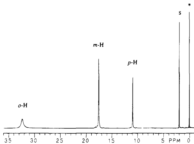
Figure 5. 1 H NMR (300 MHz) spectrum of complex 1c in (\text{CD}_3)_2\text{CO} . The peaks marked with an asterisk and S are due to HMDs and solvent proton impurities, respectively.
