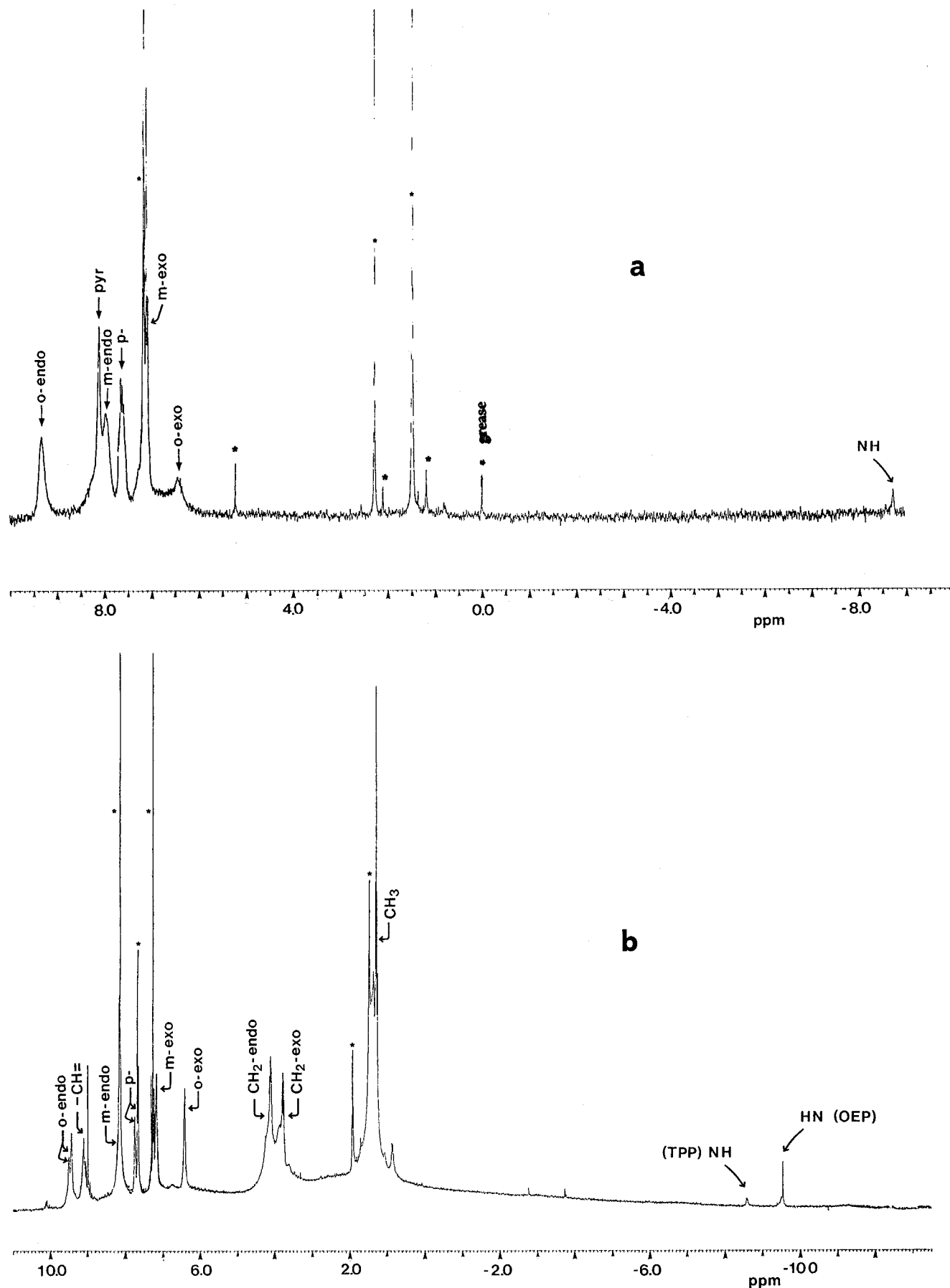
Figure 1. ^1\text{H-NMR} spectrum of (a) complex A (200 MHz, Bruker) and (b) complex B in \text{CDCl}_3 (400 MHz, Bruker). Peaks of the solvents are indicated by asterisks.
