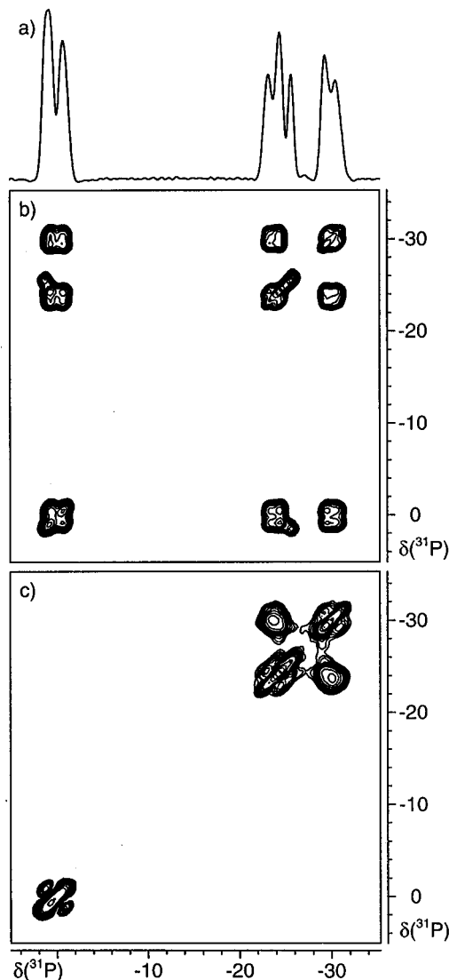
Figure 3. 31 P Solid-state NMR spectroscopy for [\text{OsH}_3(\text{dppp})_2][\text{BPh}_4] : (a) isotropic region of the conventional CP-MAS spectrum (162 MHz, \nu_{\text{rot}} = 10 kHz, \tau_{\text{contact}} = 2 ms). The four lines around \delta \approx -27 represent a resolved AB spin system with ^2J(^{31}\text{P}, ^{31}\text{P}) = 190(5) Hz. (b) 31 P spin diffusion experiment (EXSY) recorded under the same conditions as for a with a mixing time \tau_{\text{mix}} = 500 ms. (c) 31 P COSY-45 experiment showing mutual J correlations among the apical and the equatorial spins, respectively.
