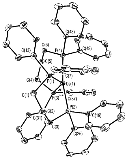
Figure 2. ORTEP view of the [\text{OsH}_3(\text{dppp})_2]^+ cation 4b .
