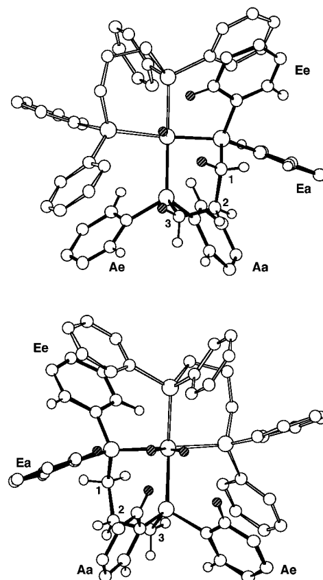
Figure 5. Model showing the locations of the H A (top) and H B (bottom) within the pentagonal bipyramidal coordination sphere of Os in [\text{OsH}_3(\text{dppp})_2]^+ ( 4b ). Hydrides and protons which are spatially close to these are shown in a shaded fashion. For clarity, one of the dppp ligands is contoured.
